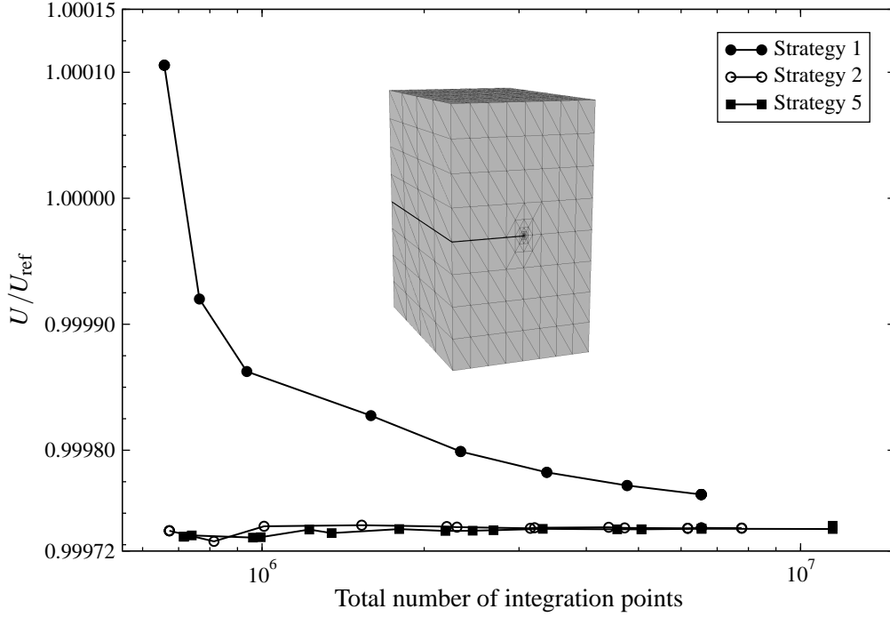
Figure 19: Convergence of strain energy with respect to the total number of integration points for elements enriched with the OD branch functions, i.e. elements with either edge or node on crack front. Semi-log scale.
