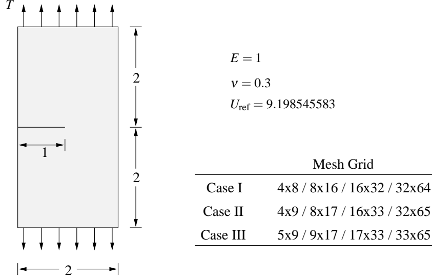
Figure 3: Geometry of problem and mesh grids for each case.
