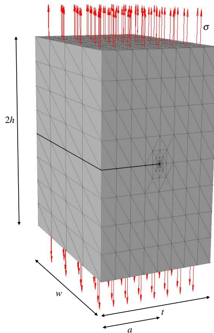
Figure 18: Edge-cracked bar: Domain dimensions, boundary conditions and mesh with localized refinement.
