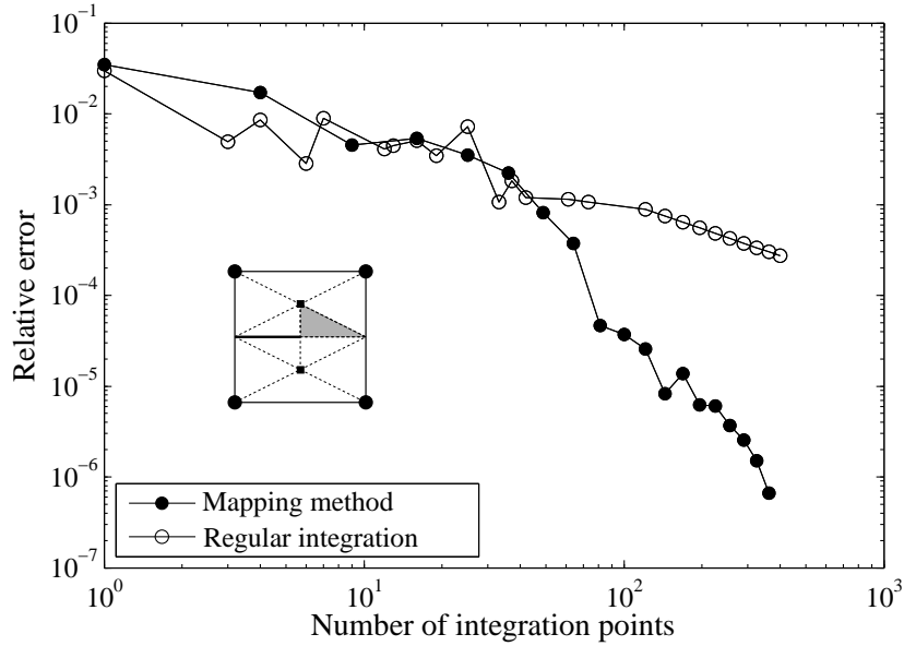
Figure 13: Convergence of the Frobenius-norm of the element stiffness matrix associated with a singular sub-triangle (shaded triangle).
