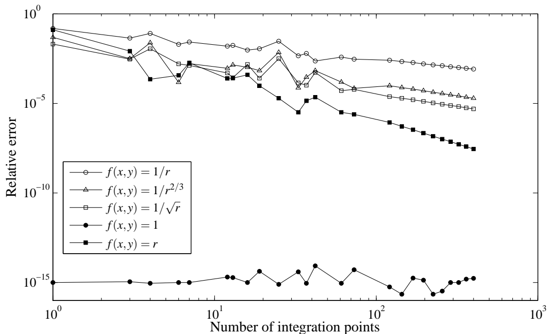
Figure 10: Convergence of numerical integration for the standard triangular integration.
