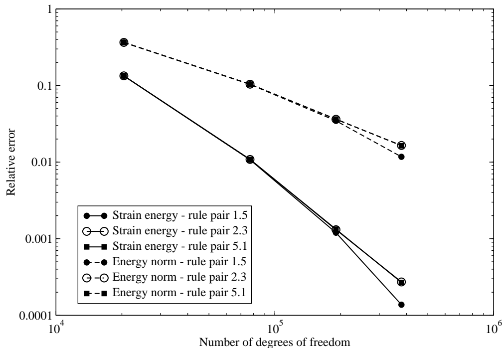
Figure 20: Convergence analysis of strain energy and energy norm with respect to the number of degrees of freedom for Mesh 1. Log-log scale. The p -version of the GFEM is used.
