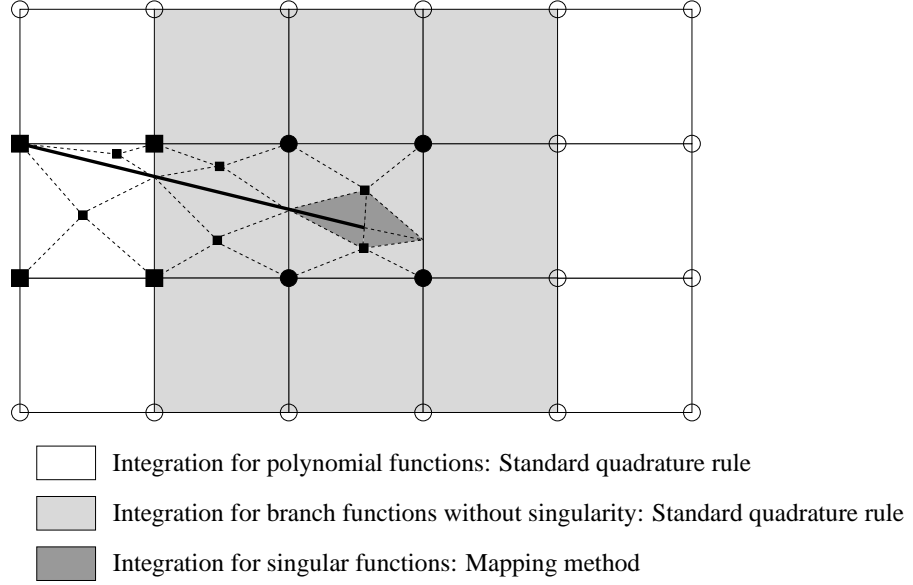
Figure 6: Numerical integration schemes with respect to enrichment functions.
