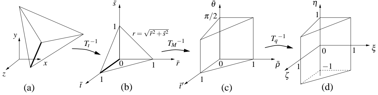
Figure 8: (a) Tetrahedron ( \Omega_{tet} ) with an edge on the singularity in the Cartesian (physical) coordinate ( x, y, z ) system, (b) tetrahedron ( \hat{\Omega}_{tet} ) in the volume coordinate ( \bar{r}, \bar{s}, \bar{t} ) system; (c) transformed prism ( \Omega_{prism} ) in the mapped coordinate ( \bar{\rho}, \bar{\theta}, \bar{t}' ) system; (d) master prism ( \hat{\Omega}_{prism} ) in the master coordinate ( \xi, \eta, \zeta ) system.
