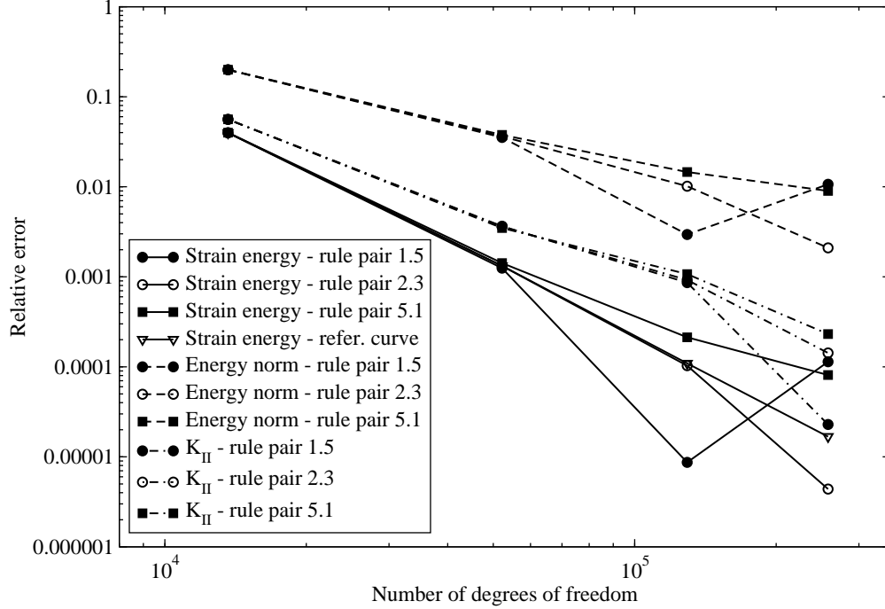
Figure 24: Convergence analysis of relative error in strain energy, energy norm and Mode II stress intensity factor with respect to the number of degrees of freedom. Log-log scale.
