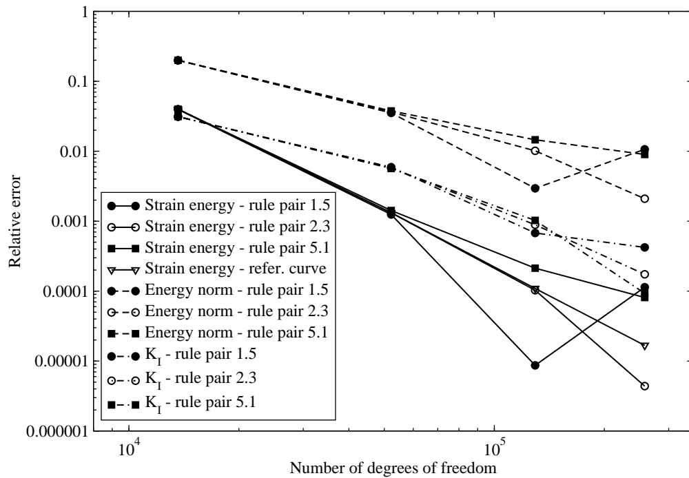
Figure 23: Convergence analysis of relative error in strain energy, energy norm and Mode I stress intensity factor with respect to the number of degrees of freedom. Log-log scale.
