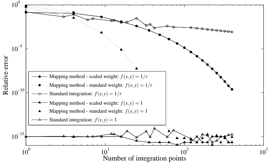
Figure 12: The effect of the scaled weight in the mapping method.
