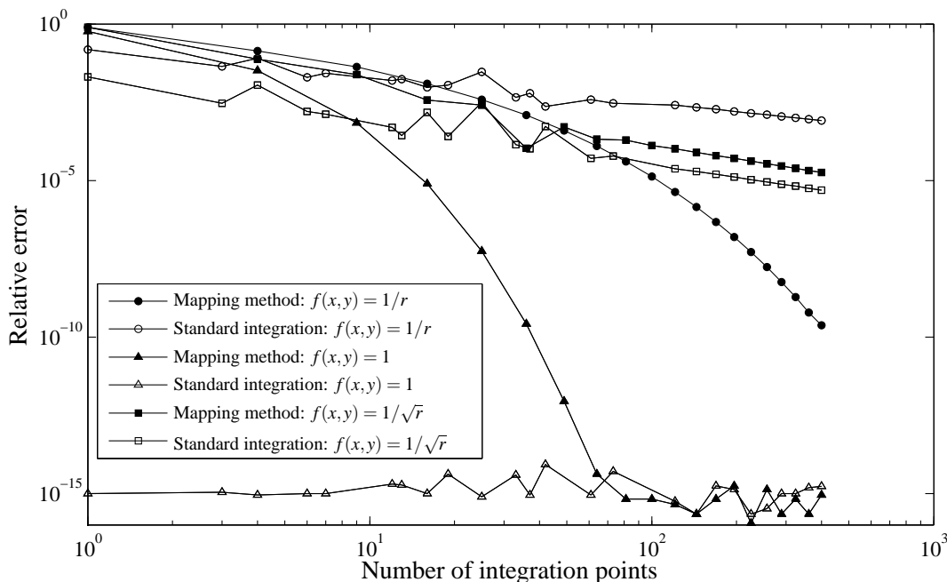
Figure 11: Comparison between the mapping method and the standard integration.
