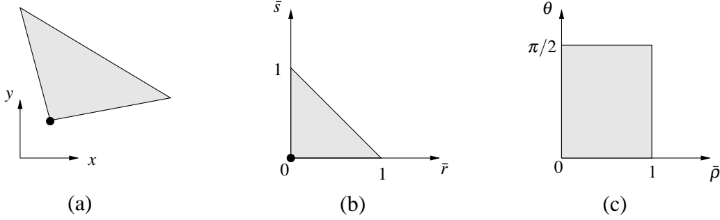
Figure 7: (a) Triangle with a node on the singularity in the Cartesian (physical) coordinate (x, y) system, (b) triangle in the area coordinate (\bar{r}, \bar{s}) system, and (c) transformed rectangle in the mapped coordinate (\bar{\rho}, \bar{\theta}) system.
