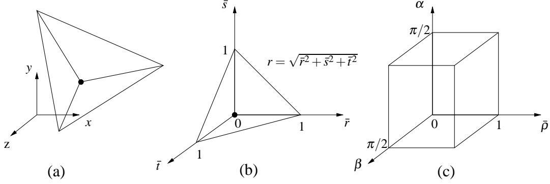
Figure 9: (a) Tetrahedron with a node on the singularity in the Cartesian (physical) coordinate (x, y, z) system, (b) tetrahedron in the volume coordinate (\bar{r}, \bar{s}, \bar{t}) system; (c) transformed hexahedron in the mapped coordinate (\bar{\rho}, \alpha, \beta) system.
