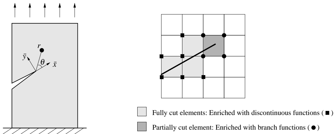
Figure 2: Enrichment cases with respect to the crack geometry.
