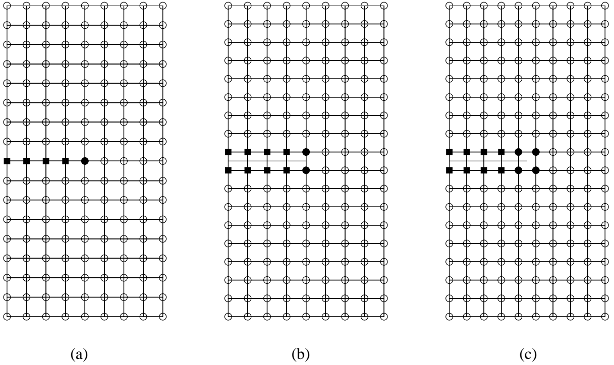
Figure 4: Finite element meshes for each case and local enrichment function types; (a) case I with the mesh grid of 8 \times 16 ; (b) case II with the mesh grid of 8 \times 17 ; (c) case III with the mesh grid of 9 \times 17 .
