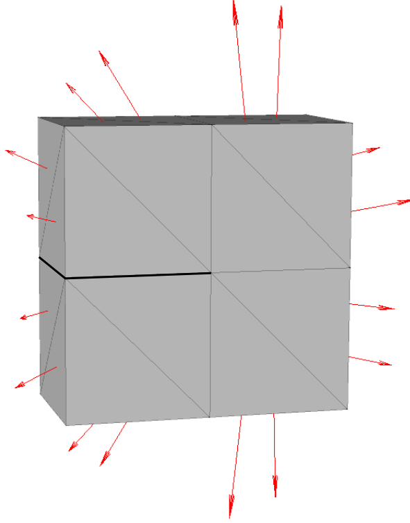
Figure 14: Edge cracked panel with mode I boundary conditions from asymptotic expansion.
