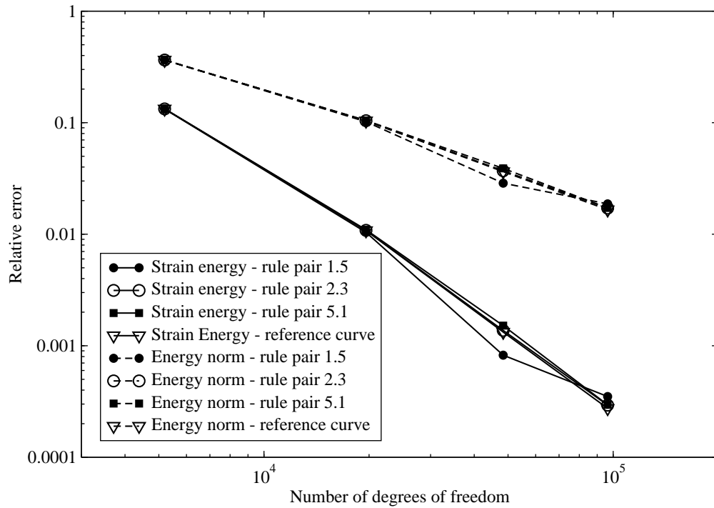
Figure 21: Convergence analysis of strain energy and energy norm with respect to the number of degrees of freedom for Mesh 2. Log-log scale.
