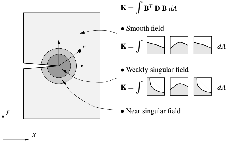
Figure 1: Example of singular behavior in linear elastic fracture mechanics problems. The notations are the following: \mathbf{K} denotes the element stiffness matrix; \mathbf{B} is the strain-displacement matrix; \mathbf{D} indicates the constitutive matrix; A is the element area.
