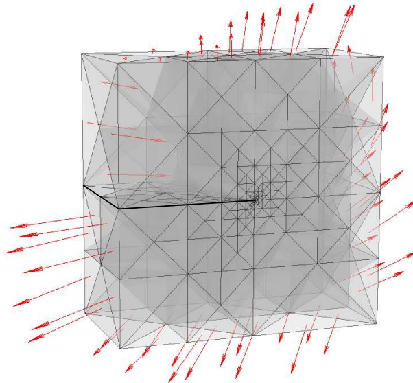
Figure 22: Edge cracked panel with Mode I and Mode II boundary conditions from asymptotic expansion.
